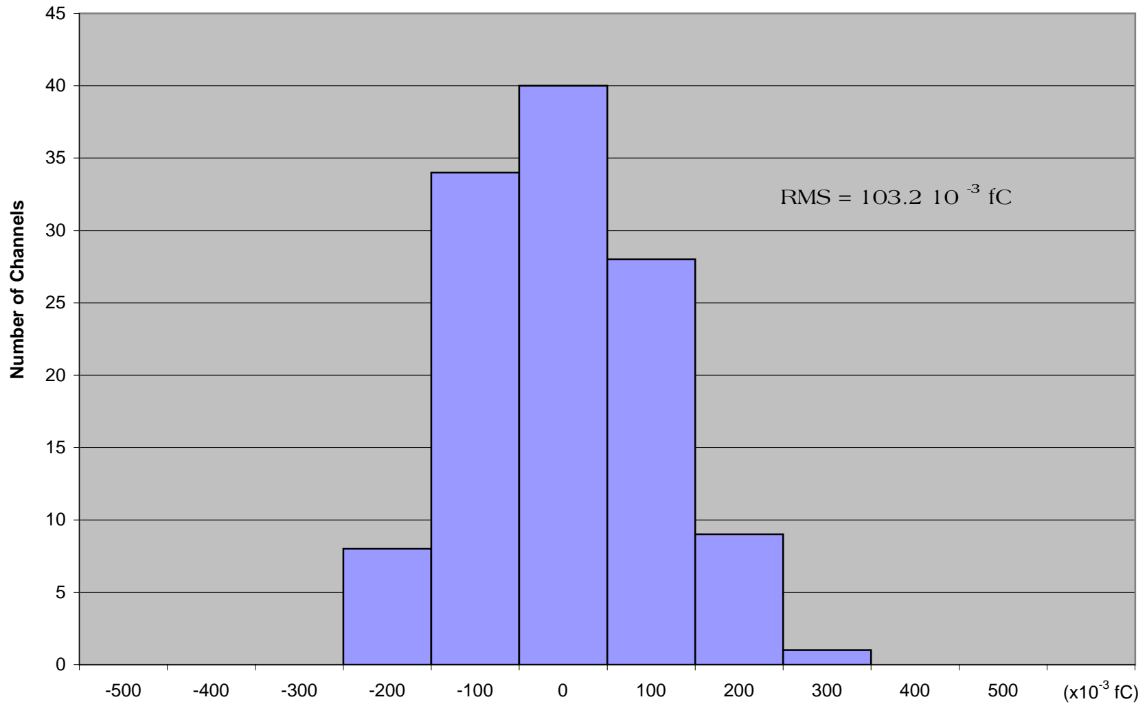
ASDBLR_00 Channel Deviation From 15 Chips Average in fC
