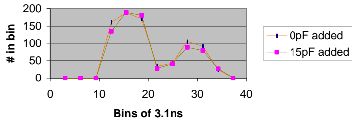
Two 4fC pulses separated by 16ns
