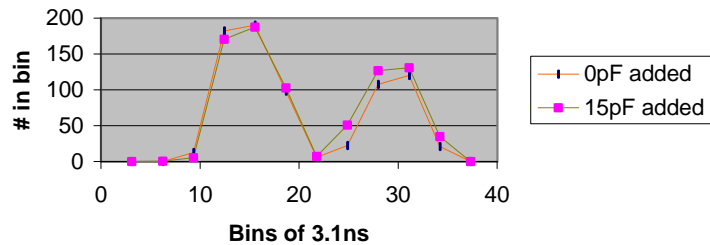
Two 4fC pulses separated by 17ns
