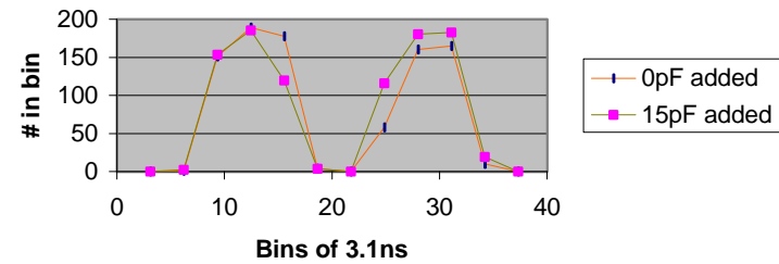
Two 4fC pulses separated by 19ns
