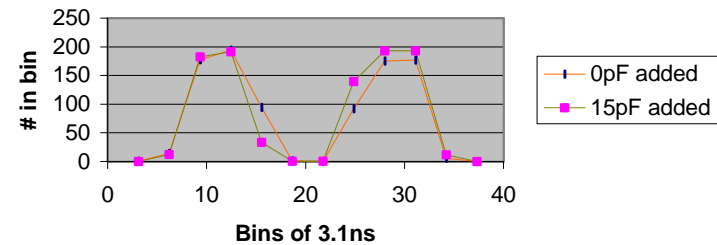
Two 4fC pulses separated by 20ns
