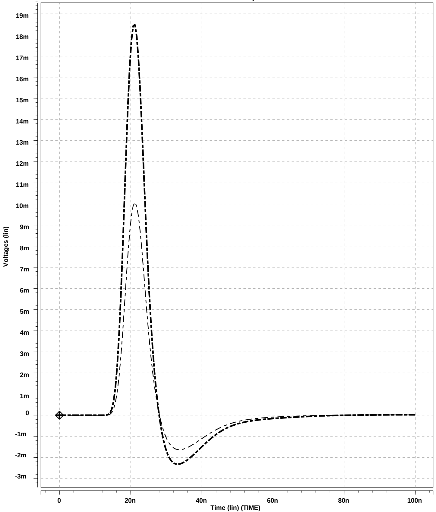
ASDBLR00 vs 02 at Track Disc Input Beta=100
