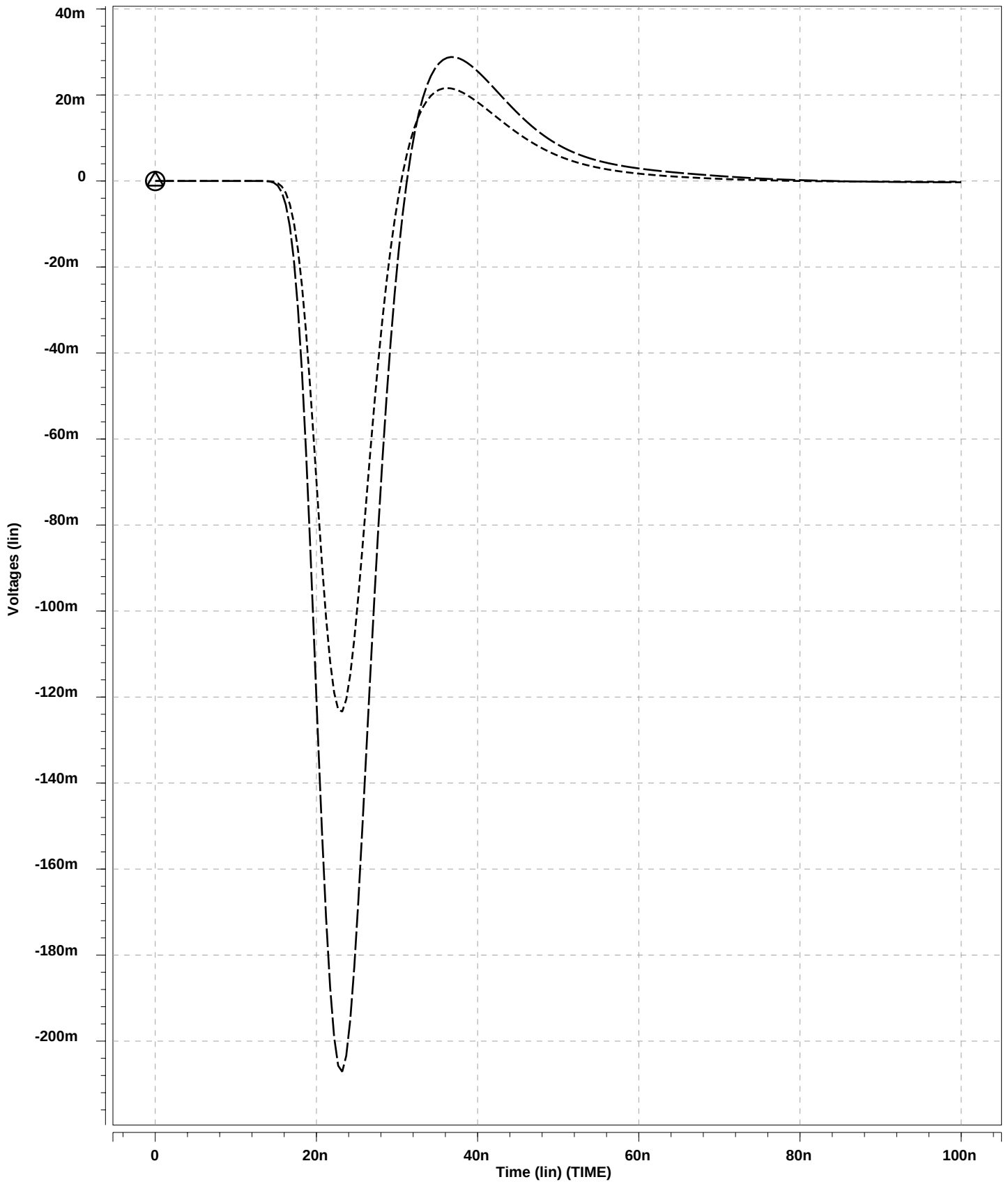
ASDBLR00 vs 02 at Track Disc Collectors Beta=100
