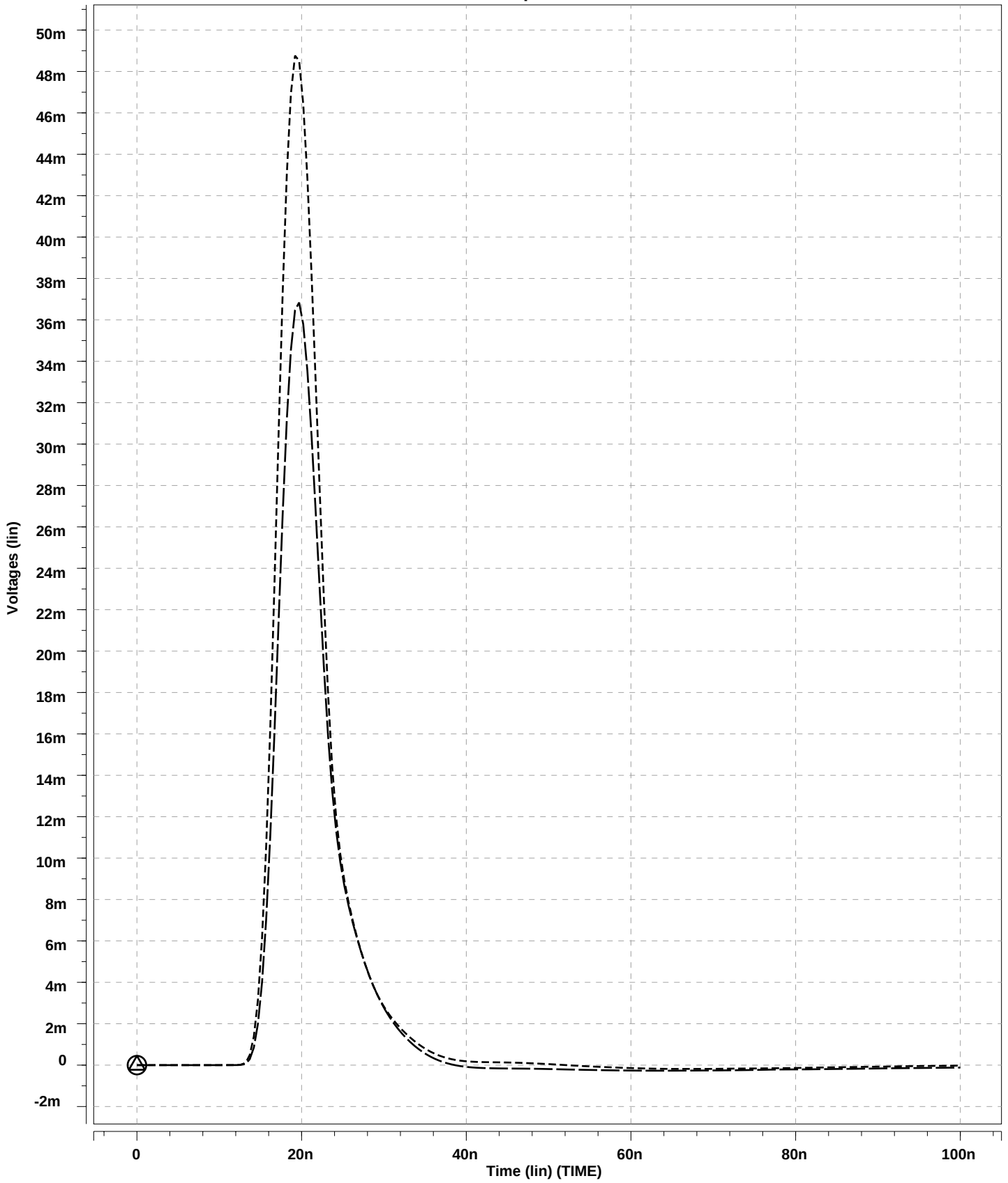
ASDBLR00 vs 02 at Shaper Out Beta=100
