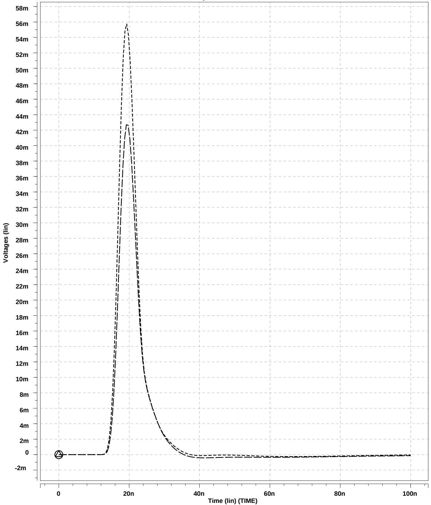
ASDBLR00 vs ASDBLR02 Shaper Out Xe 100%e 2fC Beta=250
