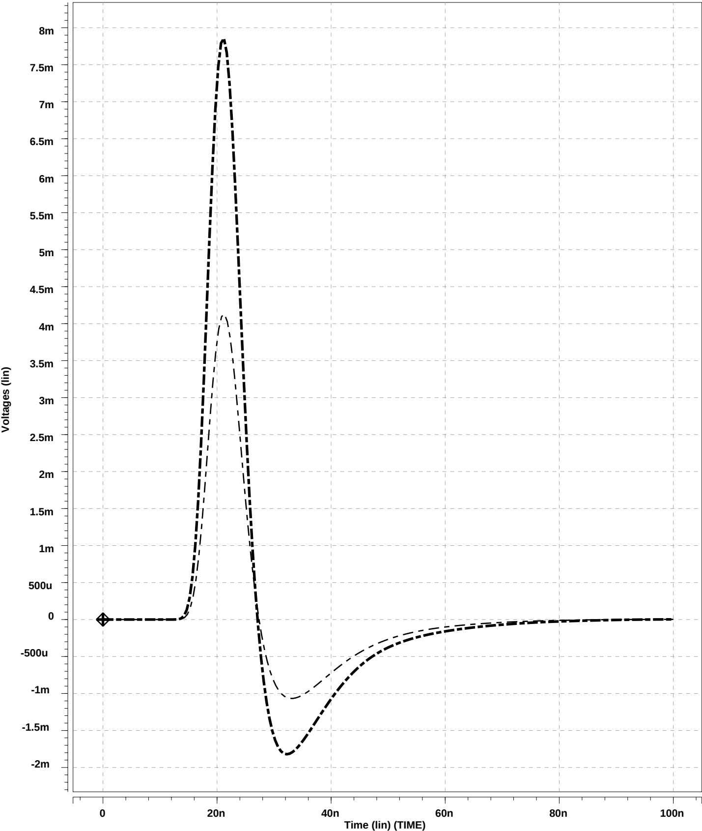
ASDBLR00 vs 02 at Track Disc Input Beta=30
