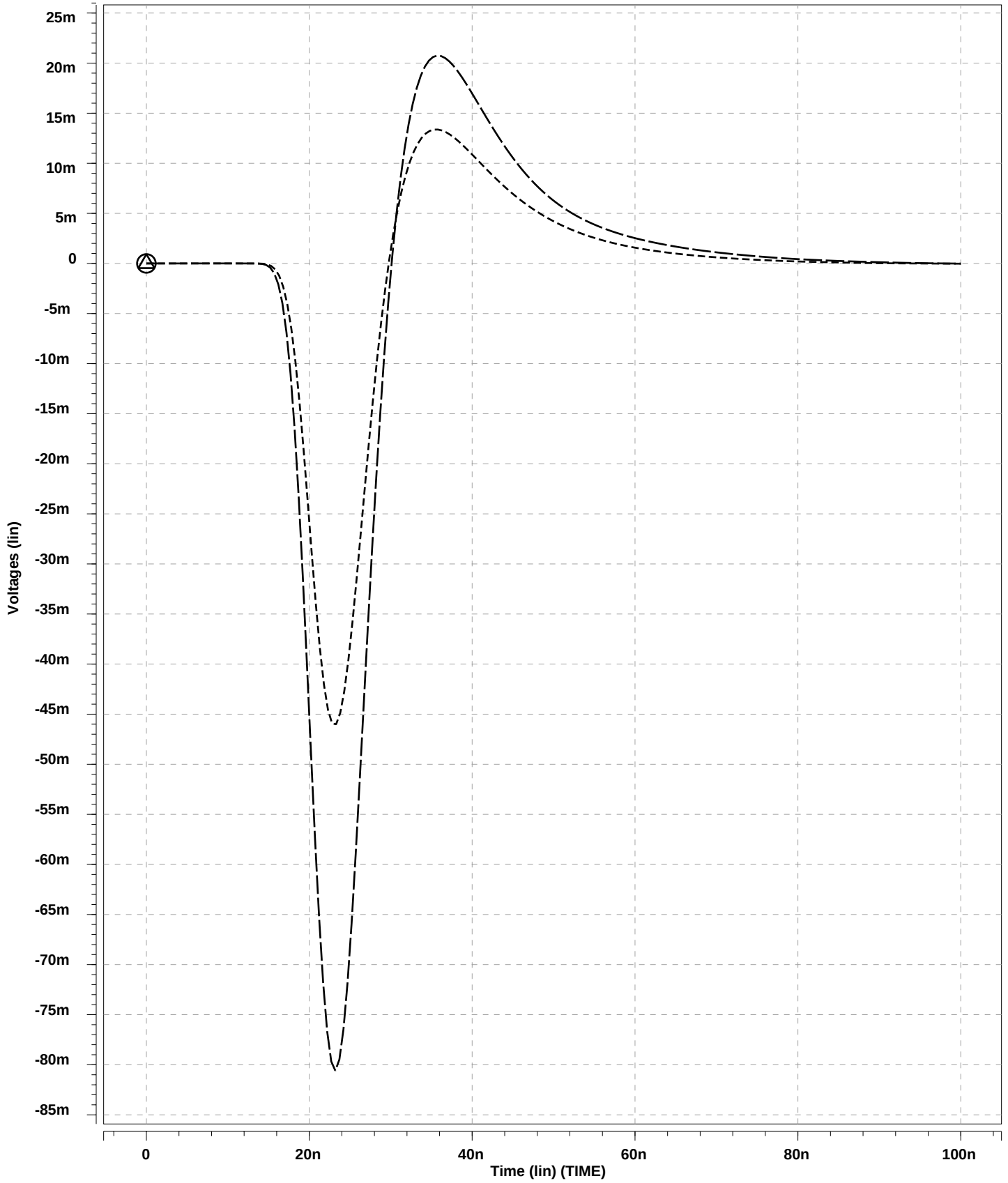
ASDBLR00 vs 02 at Track Disc Collectors Beta=30
