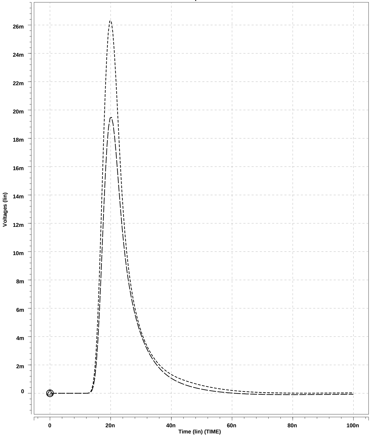
ASDBLR00 vs 02 at Shaper Out Beta=30
