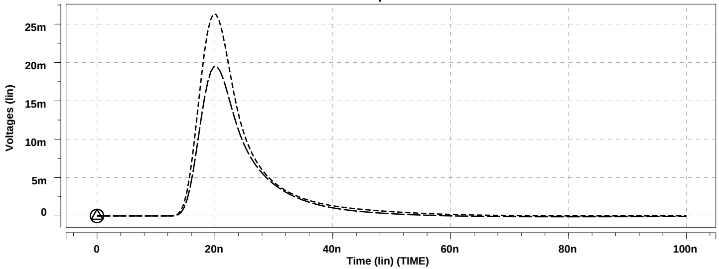
ASDBLR00 vs 02 at Track Disc Input Beta=30
