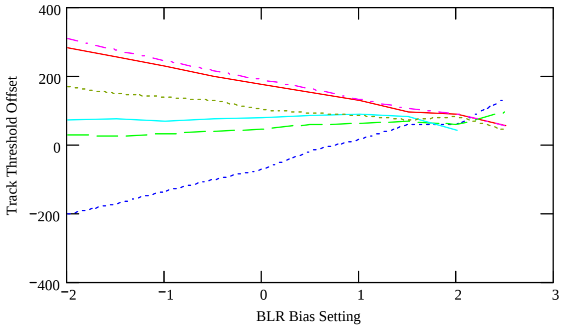
Threshold Zero point vs BLR
