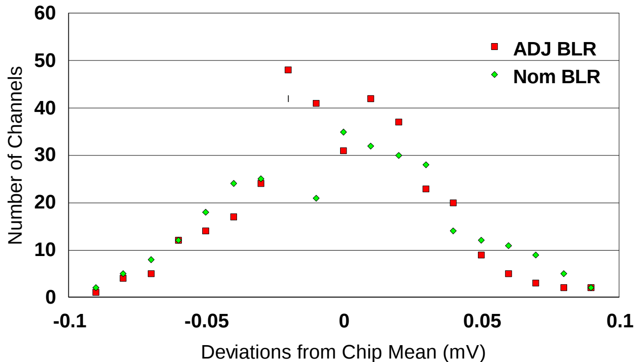
Track Threshold Deviations
