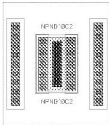
STANDARD GEOMETRY 10UM EMITTER NPN
