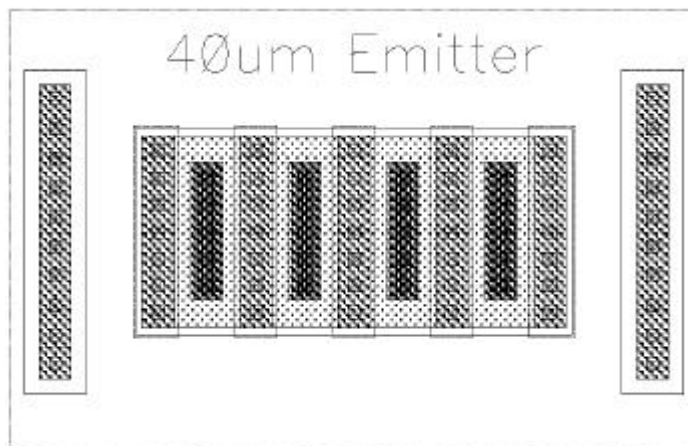
IMPROVED ROBUSTNESS, BETTER R_B EXPANDED GEOMETRY MULTI-STRIPE 4 X 10UM EMITTER NPN
