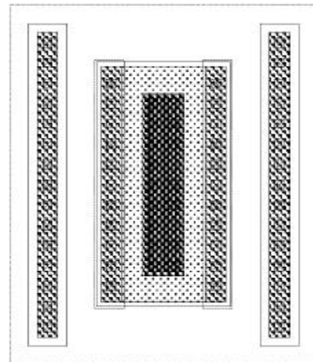
IMPROVED ROBUSTNESS, BETTER R_B EXPANDED GEOMETRY MULTI-STRIPE 4 X 10UM EMITTER NPN
