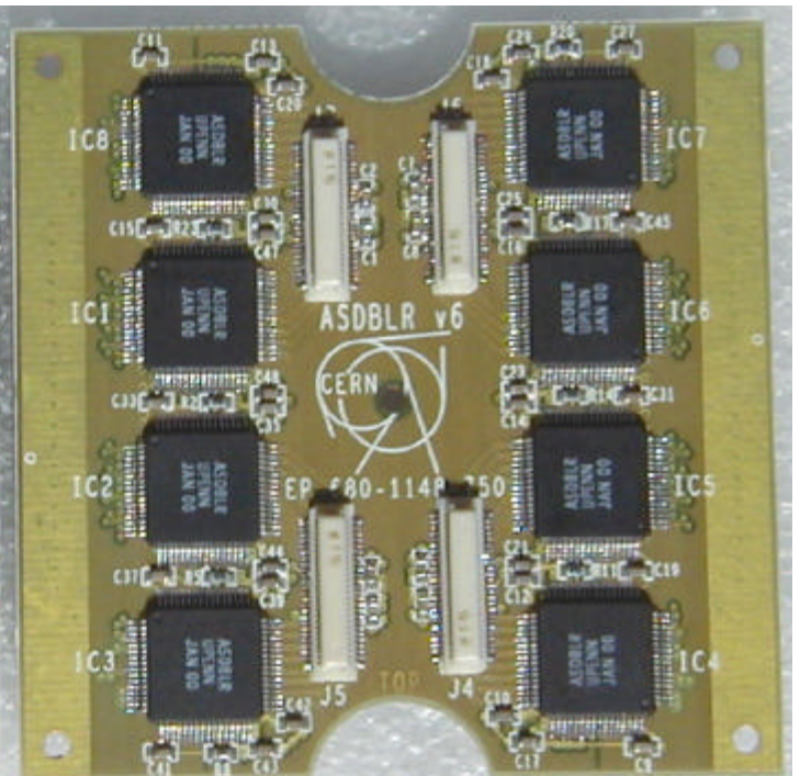
ASDBLR BOARD
