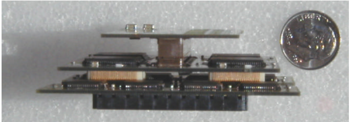
DTMROC BOARD
