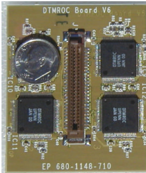
DTMROC BOARD
